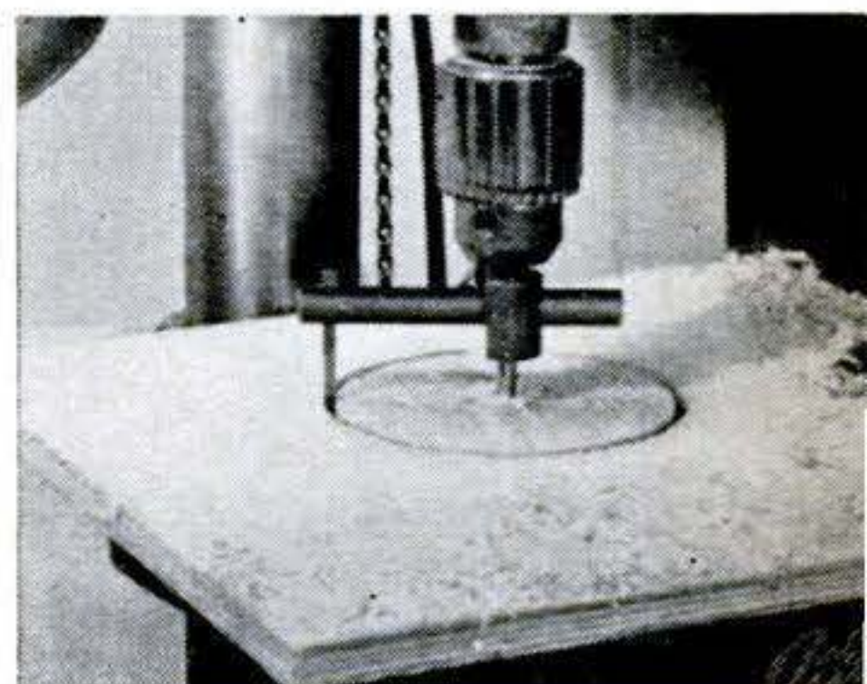
USE an adjustable circle cutter to form armhole and opening for the percolator sieve.
